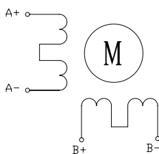
2. Bipolar (series) connection
